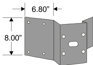
Corner Adapter for Wall Mounting Bracket CAM-WPDM-CA
