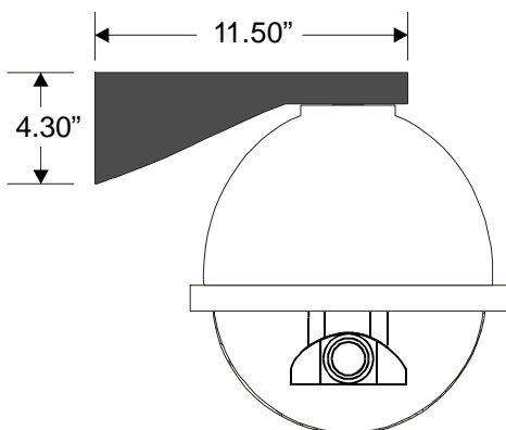
Wall Mounting Bracket CAM-WPDM-WMB
