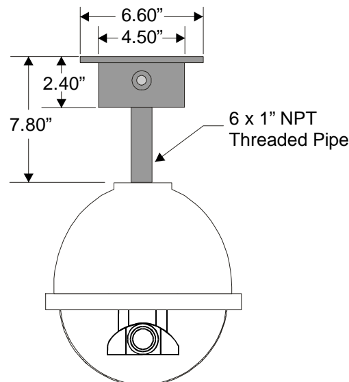
Ceiling Mounting Bracket CAM-WPDM-CMB
