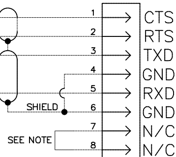
WIRING VIEW
